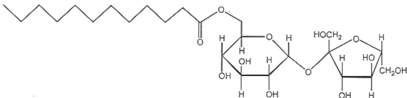
saccharose monolaurate
